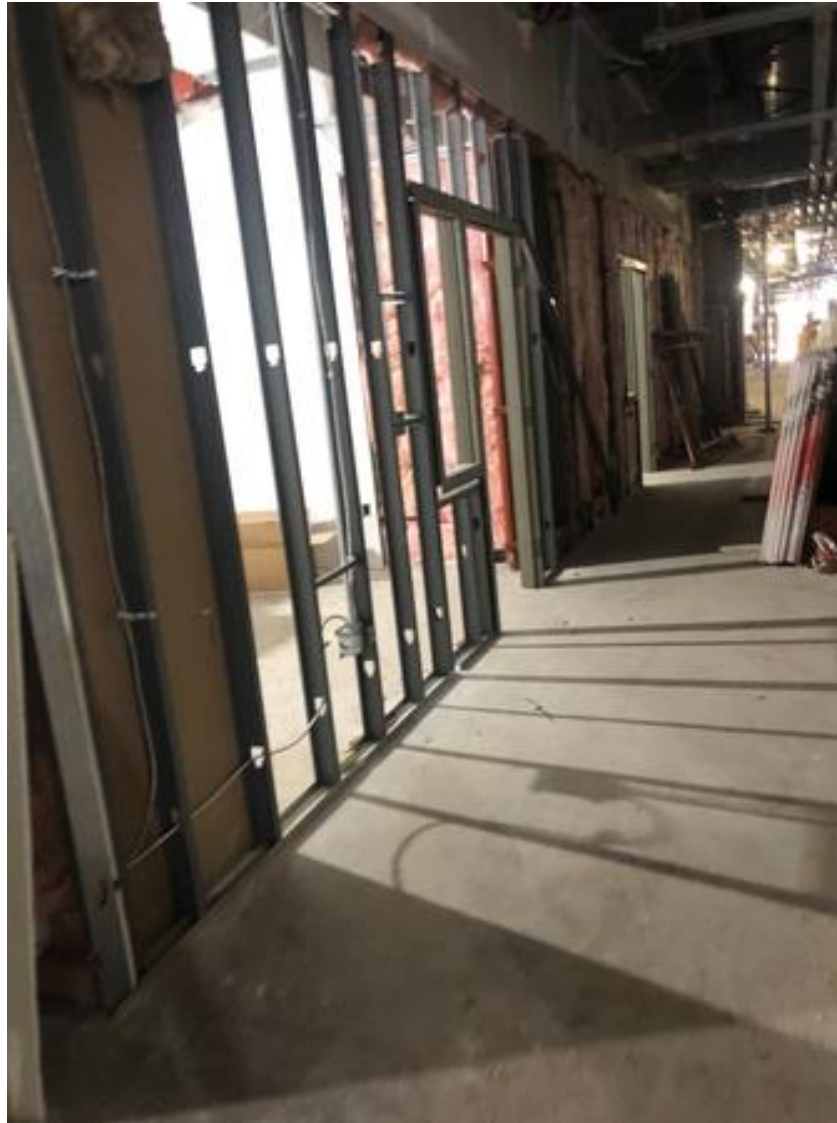
Steel stud framing and sheetrock ongoing throughout all areas
